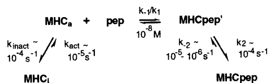
FIGURE 9: Kinetic mechanism for peptide binding to the class II MHC protein HLA-DR1. MHC i and MHC a represent inactive and active conformations of the empty protein, and MHC ep ' represents a transient peptide-bound species. Kinetic values are representative of both HA and CLIP peptide binding reactions.
