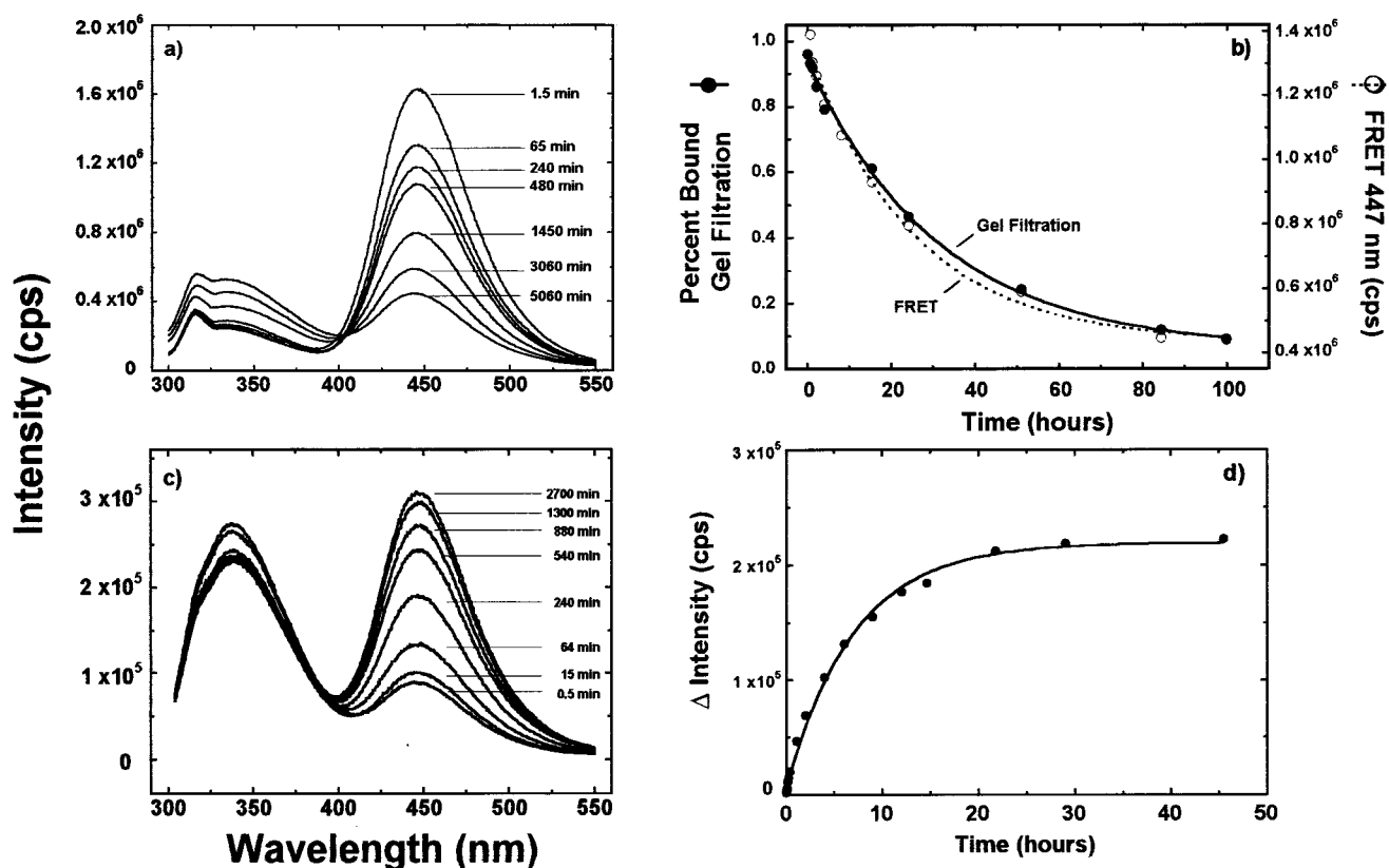
FIGURE 2: Peptide binding kinetics. (a) Dissociation assay for DR1–CLIP complex, with emission spectra recorded at 37 °C, pH 7.2, at indicated times after addition of excess unlabeled peptide (2.7 μM) to purified complex (32 nM, formed by incubation of DR1 with labeled peptide for 72 h at 37 °C with subsequent purification). Emission intensity decreases with time, indicating dissociation of labeled peptide. (b) Peak intensities for energy transfer (FRET 447 nm) from panel (a) (open symbols) plotted against dissociation time, shown along with data from conventional gel filtration assay (filled symbols) of the same dissociation reaction. The solid line represents a single-exponential fit to the FRET data ( \tau = 28 h); dashed line, gel filtration data ( \tau = 31 h). (c) Association assay for DR1–CLIP complex, with emission spectra recorded at indicated times after addition of AMCA-labeled peptide (100 nM) to empty DR1 (100 nM) at 37 °C, pH 7.2. Emission intensity at 447 nm increases with time, indicating binding of labeled peptide. (d) Change in fluorescence intensity at 447 nm plotted against association time. The solid line represents a single-exponential fit as described under Experimental Procedures. A slower binding phase ( \tau \sim 50 h) is not apparent on this scale.
