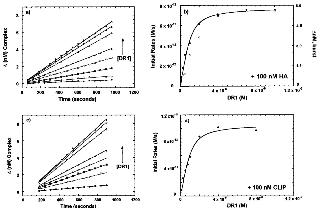
FIGURE 4: Initial rates with varying concentration of MHC. (a) Dependence of peptide binding kinetics on DR1 concentration, with 100 nM AMCA-HA and varying DR1 concentrations [(●) 50 nM, (○) 100 nM, (■) 250 nM, (□) 500 nM, (▲) 1 \mu M, (△) 2 \mu M, (◆) 4 \mu M, (◇) 7 \mu M, (▼) 10 \mu M]. Changes in concentration relative to an extrapolated time zero value are shown (see Experimental Procedures for details). (b) Initial rate of peptide binding plotted against DR1 concentration. The amount of complex formed in the burst phase for each association reaction is shown as (○). (c, d) Same for CLIP; DR concentrations are (●) 100 nM, (○) 250 nM, (■) 500 nM, (□) 750 nM, (▲) 1 \mu M, (△) 2 \mu M, (◆) 4 \mu M, (◇) 8 \mu M.
