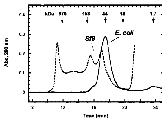
FIGURE 7: Monomeric DR1 produced in E. coli . Comparison of gel filtration profiles for DR1 produced in baculovirus-infected insect cells (dashed line) and monomeric DR1 refolded in vitro from subunits expressed in E. coli (solid line). The arrows above the plot indicate the positions of molecular weight standards. The species eluting at times > 20 min represent buffer components in the insect cell preparation.
